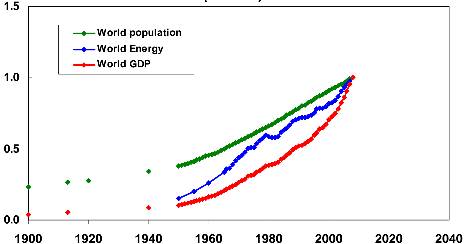
World Population, GDP, Energy 1900-2008 (2008=1)
